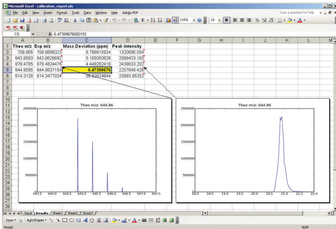
Figure 9 Instrument Calibration Quality Control Report. An .mz script is used to automatically generate a spreadsheet report that indicates mass errors (in ppm) for a set of standard peptides. Images of the precursor isotope distribution and reconstructed ion chromatogram are embedded within the report for rapid confirmation of mass spectrometry and chromatographic performance.
